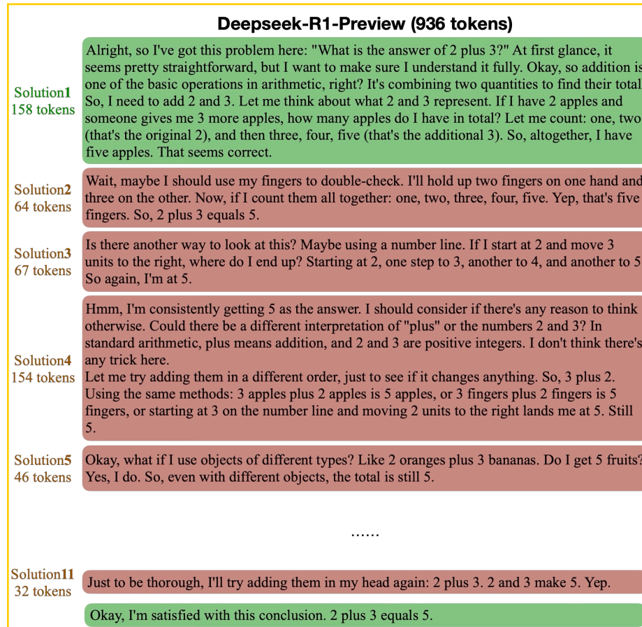
Figure 8: Deepseek-R1-Preview response for the query "What is the answer of 2 plus 3?"
